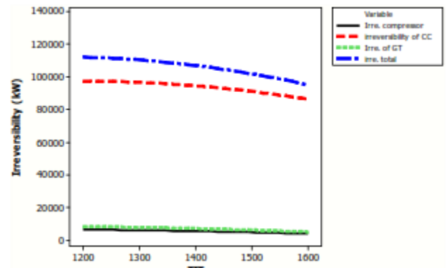
Fig. 3 Irreversibility rates of components verses turbine inlet temperature
