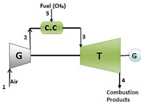
Fig. 1 Gas Turbine Power Plant
