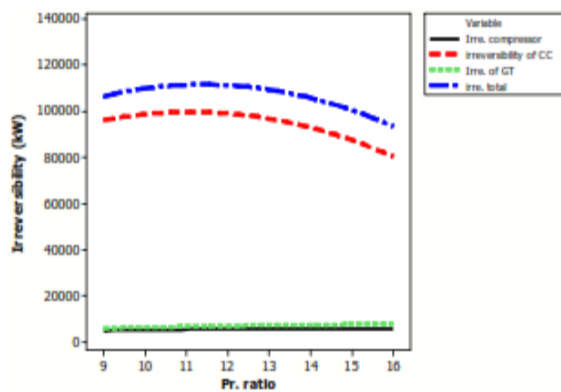
Fig. 1 Irreversibility rates of components verses pressure ratio
